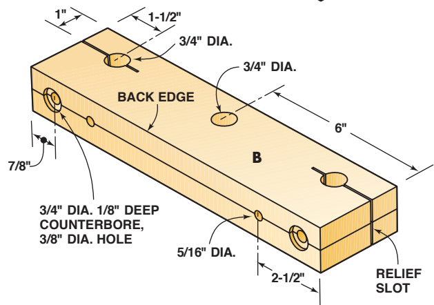
Fig. E Lower Clamp Block
