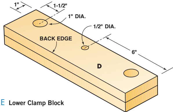
Fig. D Lower Slide Block
