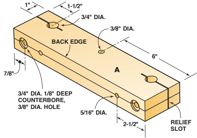
Fig. C Upper Slide Block
