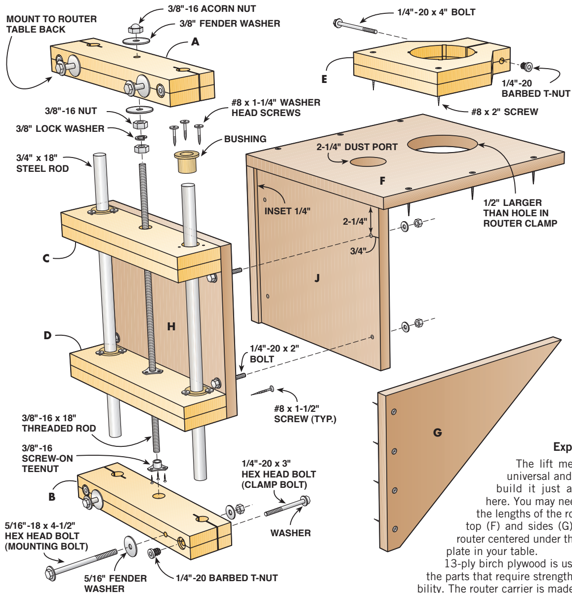
Fig. A Exploded View
